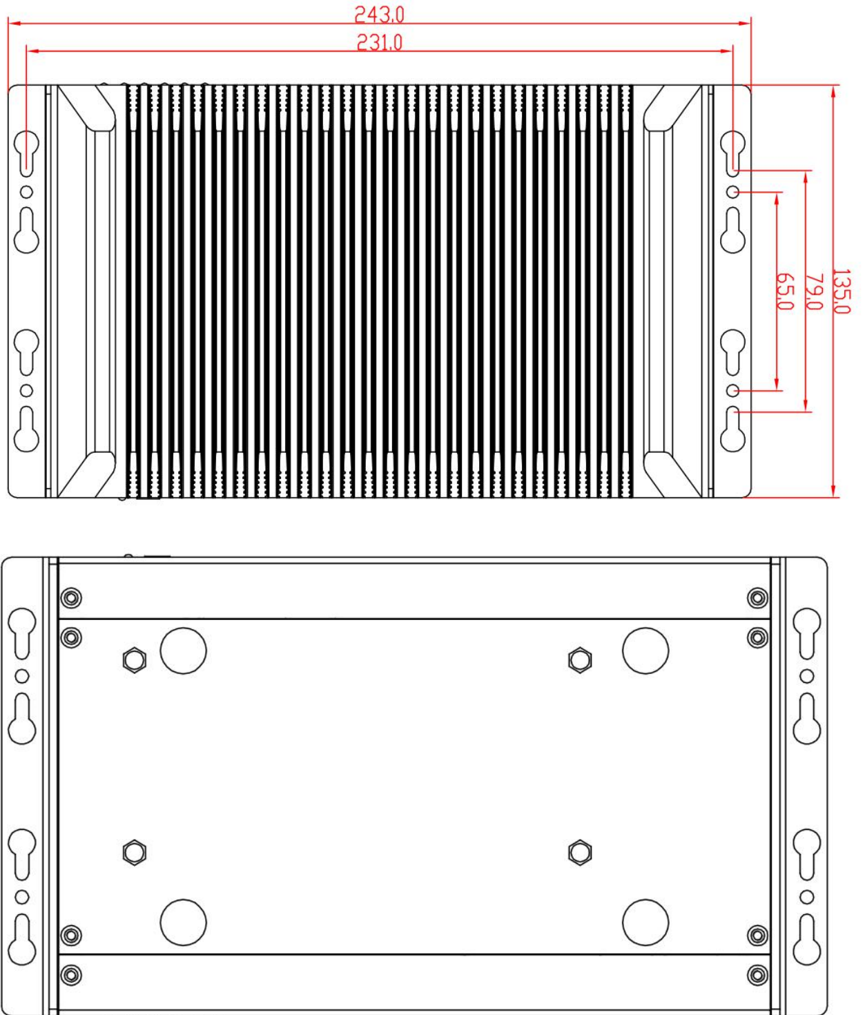
Figure 1.7 NIS-S990B Upper and lower cover mechanical dimension drawing
