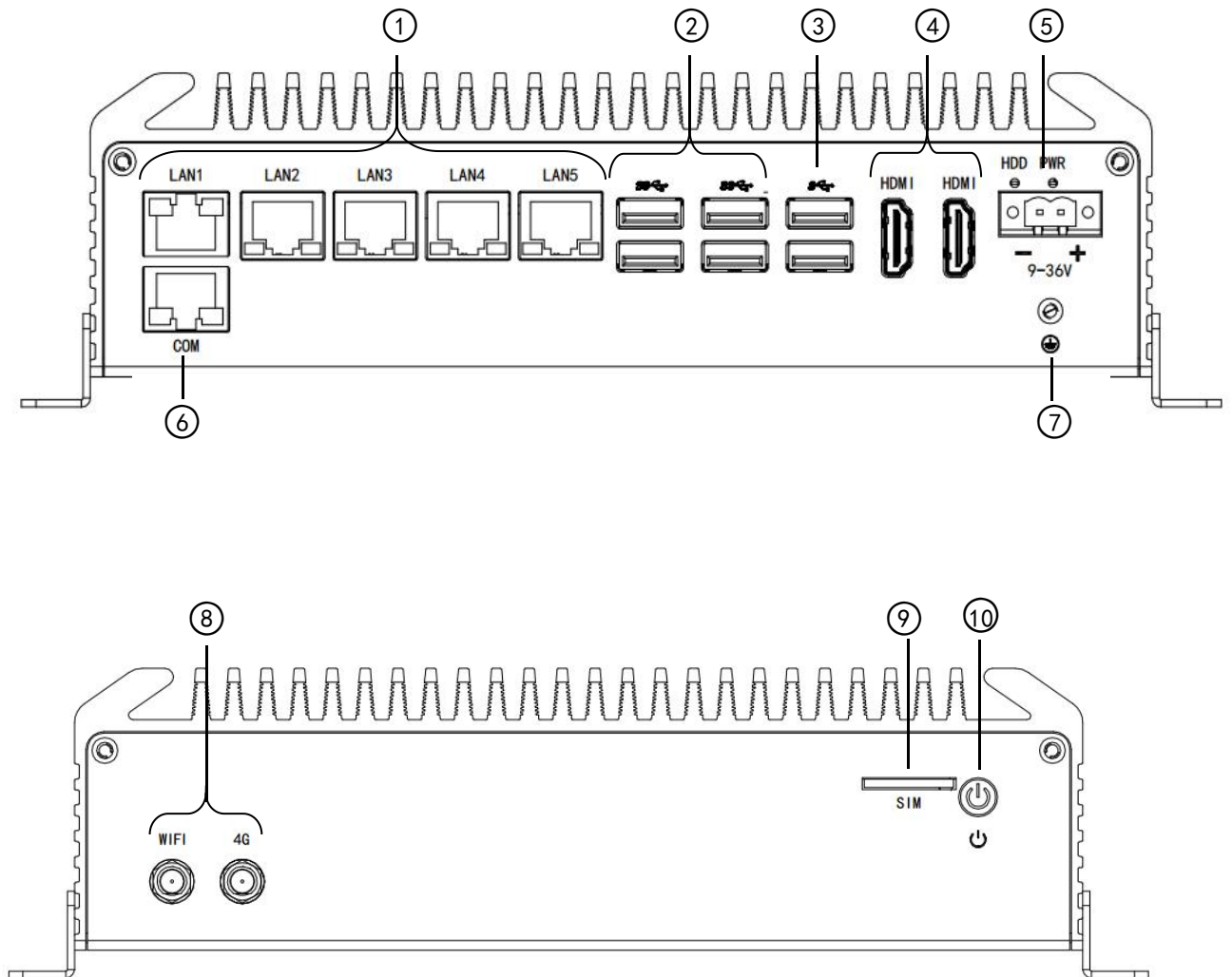
Figure 2.1.3 NIS-S990B mechanical dimension drawing
