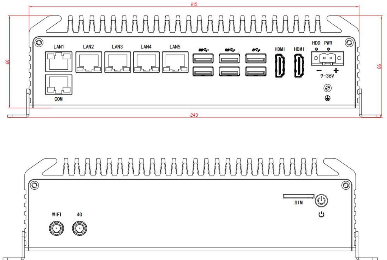
Figure 1.8 NIS-S990B Front+Side cover mechanical dimension drawing
