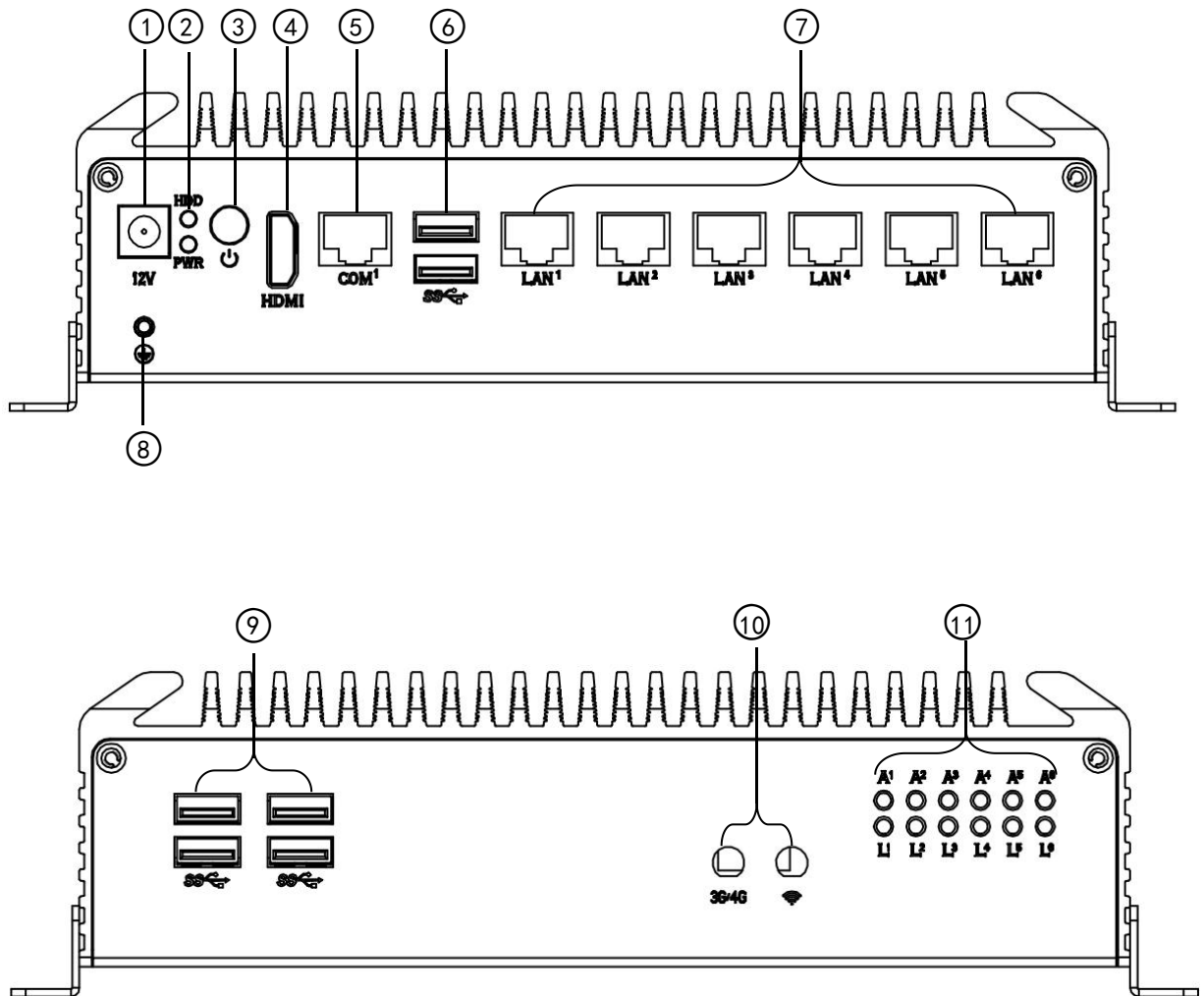
Figure 2.1.3 NIS-S990 mechanical dimension drawing
