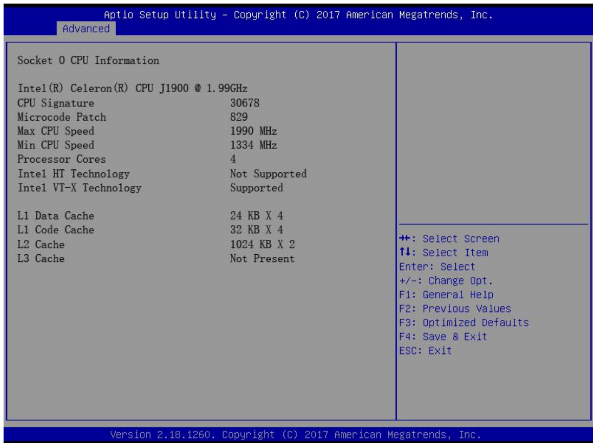
Figure 3.3.2 CPU Configuration
