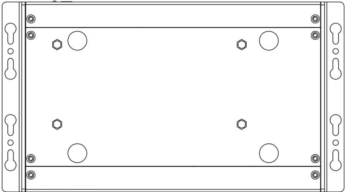
Figure 1.7 NIS-S990 Upper and lower cover mechanical dimension drawing
