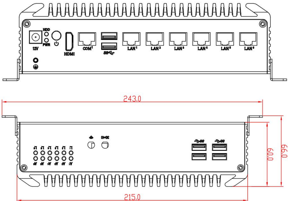
Figure 1.8 NIS-S990 Front+Side cover mechanical dimension drawing
