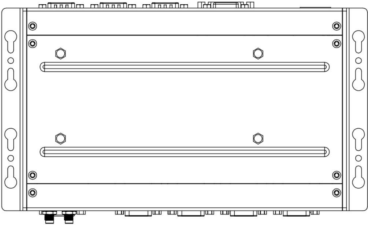
Figure 1.7 NIS-S991 Upper and lower cover mechanical dimension drawing
