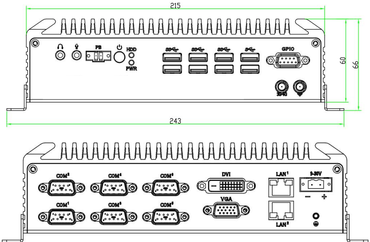
Figure 1.8 NIS-S991 Front+Side cover mechanical dimension drawing
