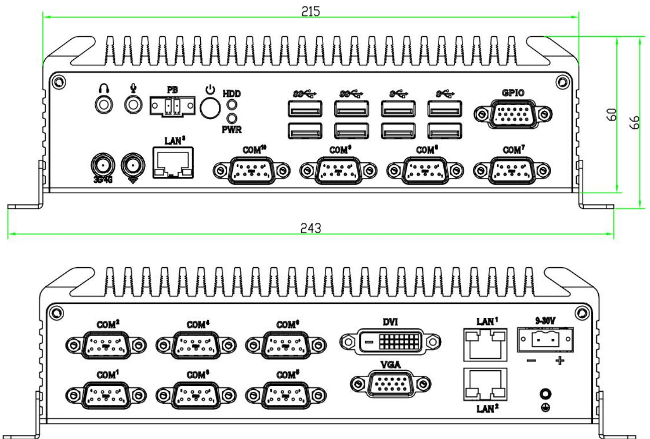
Figure 1.8 NIS-S993 Front+Side cover mechanical dimension drawing
