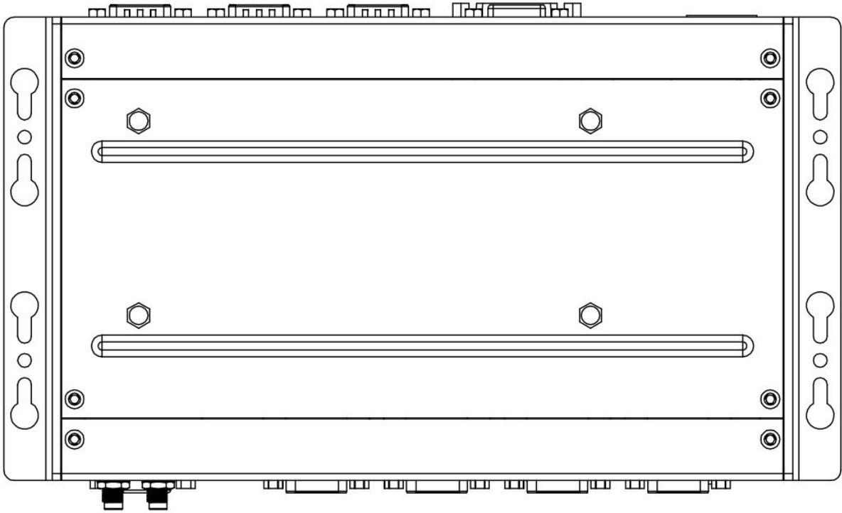
Figure 1.7 NIS-S993 Upper and lower cover mechanical dimension drawing
